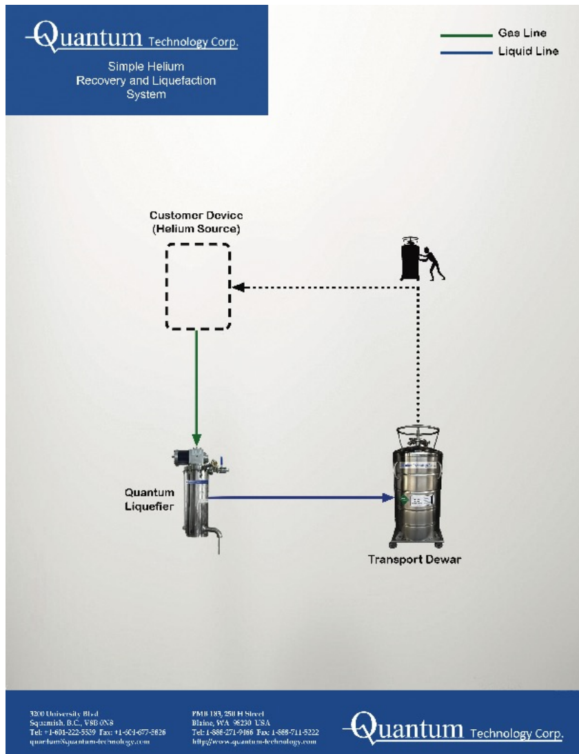
Figure 1. QHRLS - DR – Helium direct recovery system
